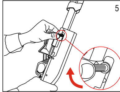
5) Turn ramp lever down.
